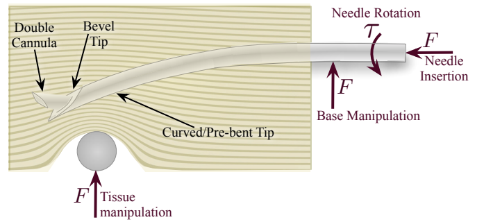
Fig. 2: Several different methods of needle steering have been proposed in the literature: Asymmetry-based steering uses the forces generated at the tip during insertion to bend the needle. The tip curvature can be either constant or variable using multiple concentric cannulas. Base manipulation bends the needle by applying a force perpendicular to the insertion direction. Tissue manipulation can move the targets and obstacles into and out of the needle’s path, respectively. Each of these methods are conceptually independent, but may be combined, thereby increasing control authority over the needle trajectory.
