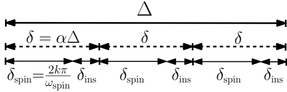
Fig. 4. The time duration \Delta is split into three intervals of duration \delta each for \alpha = \mathbf{h}[\kappa] = 1/3 . Each interval is then composed of two intervals: (i) a spin interval of duration \delta_{\text{spin}} = (2k\pi/\omega_{\text{spin}}) , k \in \mathbb{Z} in which the needle is both inserted and rotated, and (ii) an insertion interval of duration \delta_{\text{ins}} in which the needle is only inserted without any rotation.
