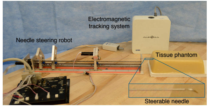
Fig. 5. Our needle steering system consists of a needle steering robot, a pre-bent, bevel-tip steerable needle, and an electromagnetic tracking system. We present details of the hardware system in Sec. VI. We performed experiments using a tissue phantom (shown here) and porcine tissue ex vivo .
