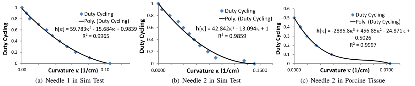
Fig. 7. Characterization of the relationship \alpha = \mathbf{h}[\kappa] (Eqn. (3)) for Needle1 (0.92 mm diameter) and Needle 2 (0.88 mm diameter) in Sim-Test tissue phantom and porcine tissue ex vivo.
