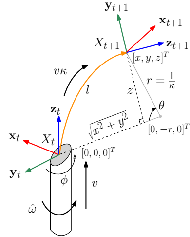
Fig. 3. Local coordinate frame X_t attached to the needle tip and a point in \mathbb{R}^3 : [x, y, z]^T defined in the local coordinate frame. The needle is inserted along the z -axis, and the needle rotates around a line parallel to the x -axis and passing through the point [0, -r, 0]^T . The variable curvature circular arc followed by the needle (shown in orange) is parameterized as a triplet [l, \phi, r] .
