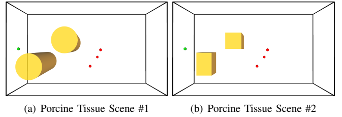
Fig. 11. We perform targeting experiments in a porcine tissue sample ex vivo. We assume that the approximately cuboidal workspace contains virtual obstacles (shown in yellow) for planning purposes. The insertion location of the needle is marked in green and the needle is inserted into the face of the tissue sample (pointing into the plane of the page). We selected 3 randomly chosen targets (shown in red) in the workspace that are located at insertion depths ranging from 10 cm to 11 cm from the insertion face.
