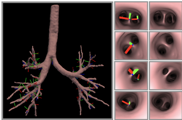
Fig. 5. A 3D model of the airways segmented from a preoperative CT scan where each bifurcation is tagged with a 6 DoF pose (visualized using the coordinate frames) (left). Simulated bronchoscopy views from inside the airways with the bifurcation tags (middle), and the same views as they exist in the dataset without explicit tags (right).
